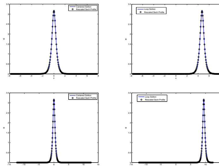
FIGURE 8. Comparison of the standing waves (solid line) localized in the central link (left) and in one of the rings (right) to the rescaled solitary wave profile (dots) for L = \pi/2 (top) and L = 2\pi (bottom) for \Lambda = -10.0 .
