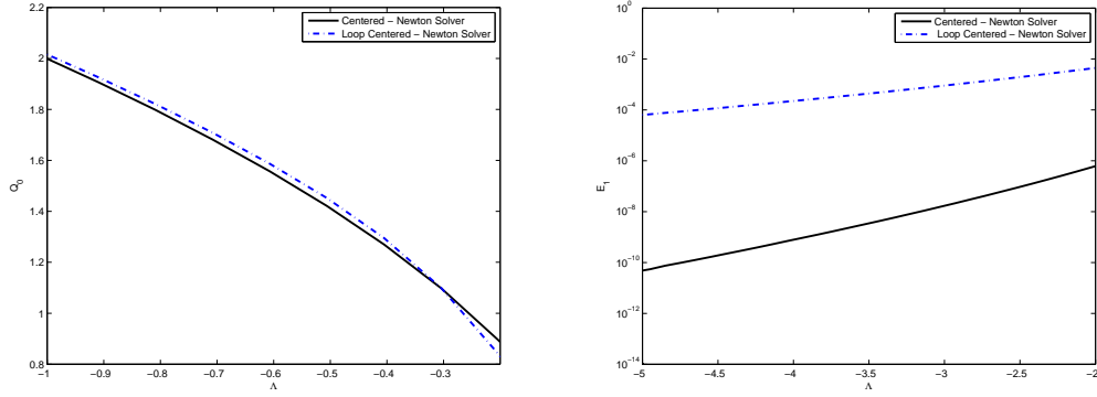
FIGURE 10. Left: comparison of the bifurcation diagram for positive solutions localized in the central link and in one of the two rings for L = 2\pi . Right: the second eigenvalue of the linearization operator L_+ associated with the two positive solutions plotted with respect to \Lambda in a semilog plot.
