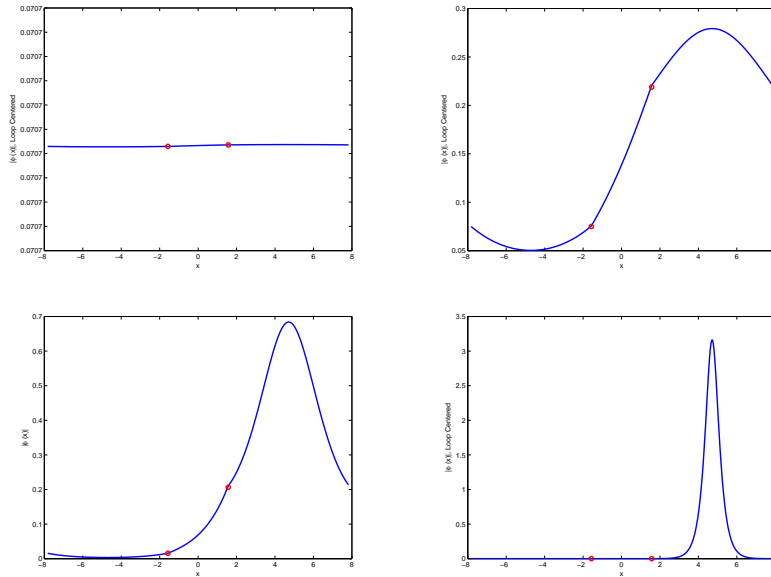
FIGURE 7. The same as in Figure 6 but for the initial iterate being localized on the right ring.
