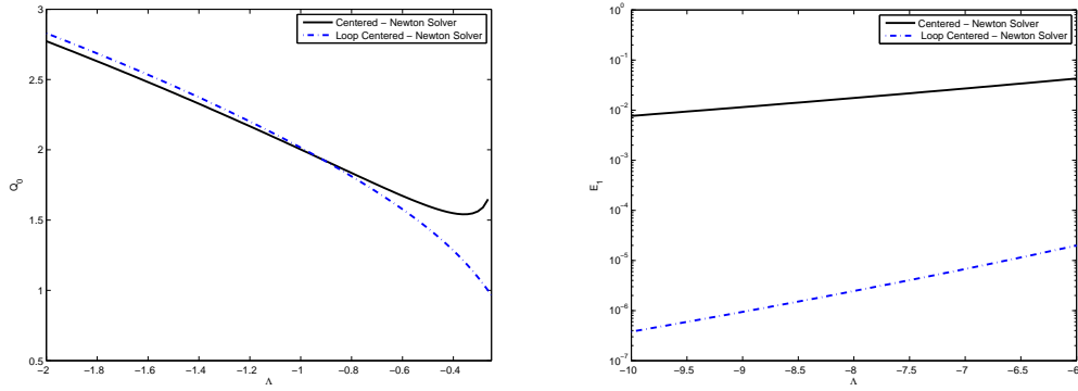
FIGURE 11. The same as Figure 10 but for L = \pi/2 .
