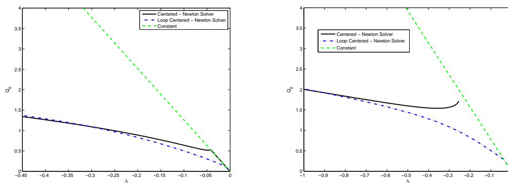
FIGURE 9. The bifurcation diagram for two positive solutions localized in the central link and in one of the two rings as well as for the constant solution for L = 2\pi (left) and L = \pi/2 (right).
