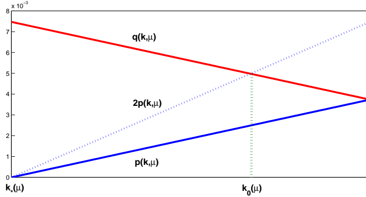
FIGURE 5. The graphs of p (solid blue), q (solid red), and 2p (dashed blue) versus k in (k_*(\mu), 1) for \mu = 2 and L = \pi . The dotted line shows a graphical solution of the equation q = 2p at k_0(\mu) .
