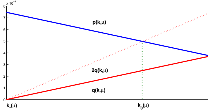
FIGURE 4. The graphs of p (solid blue), q (solid red), and 2q (dashed red) versus k in (k_*(\mu), 1) for \mu = 2 . The dotted line shows a graphical solution of the equation p = 2q at k_0(\mu) .
