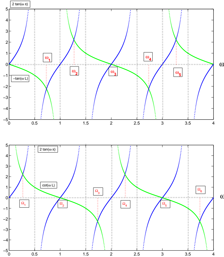
FIGURE 2. Graphical solutions of the dispersion relations (2.2) (top) and (2.3) (bottom) for L = \frac{\pi}{2} .
