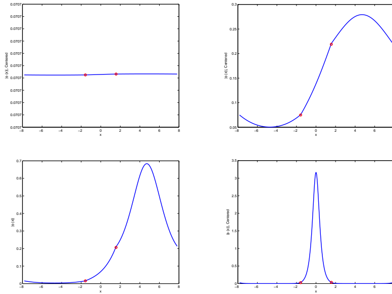
FIGURE 6. Solutions of the stationary NLS equation (1.5) for L = \pi/2 , when the initial iterate is localized on the central link, for \Lambda = -0.01 (top left), \Lambda = -0.1 (top right), \Lambda = -1.5 (bottom left), and \Lambda = -10.0 (bottom right). The values at \pm L are marked with a red circle.
