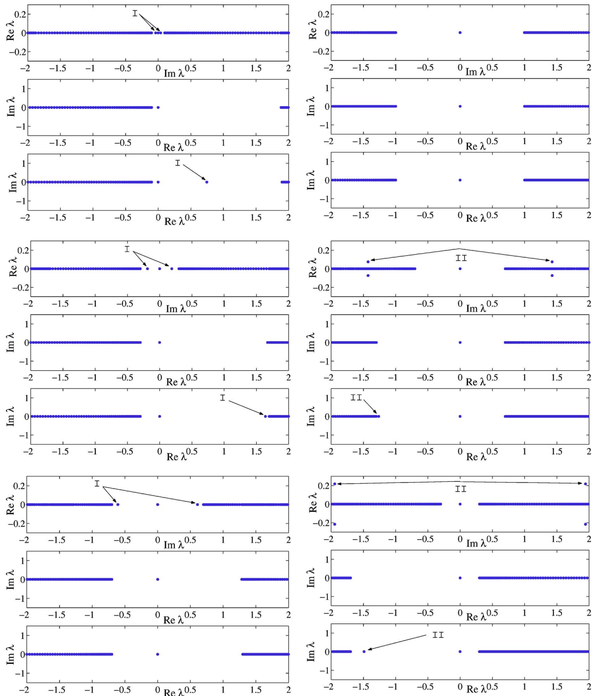
FIG. 1. (Color online) Eigenvalues and instability bifurcations for the operators L , H_+ , and H_- in Eqs. (27)–(29). The parameter values are \Omega = -0.9 (top left), \Omega = -0.7 (top right), \Omega = -0.3 (middle left), \Omega = 0.0 (middle right), \Omega = 0.3 (bottom left), and \Omega = 0.7 (bottom right).
