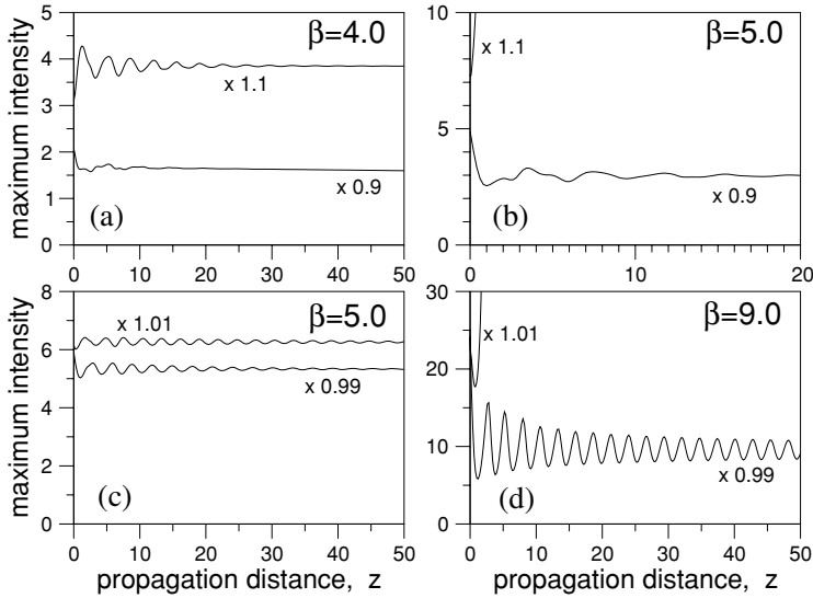
Figure 2. Results of numerical simulations of the soliton dynamics in the scalar case. The initial stationary solution is perturbed by two amplitude scalings (indicated in the graphs): one is higher and the other one is lower than the unity. Shown is the maximum soliton intensity versus the propagation distance.
