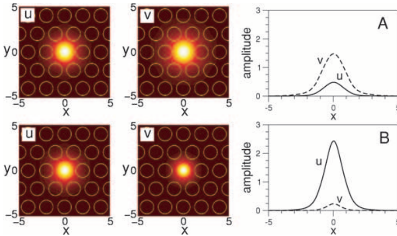
Figure 3. Examples of the two-component stationary solutions of the model (2) for vector solitons in PCFs. Two cases correspond to the points A ( \beta = 5 , \gamma = 4 ) and B ( \beta = 5 , \gamma = 8 ) in the existence domain shown in Figure 4 for \mu = 2 . In each column both components are shown in the plane (x, y) , together with a one-dimensional x -cutoff profile to compare the field amplitudes.
