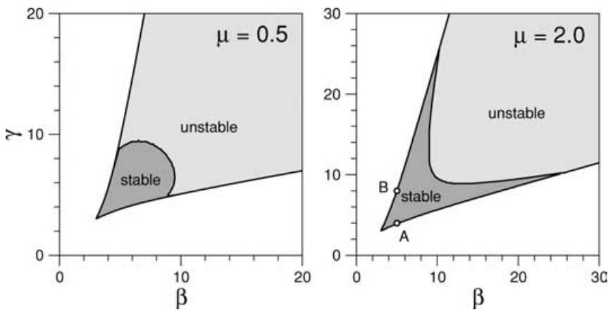
Figure 4. Existence domain for the vector solitons in PCF in the plane (\beta, \gamma) , shown at two values of the coupling parameter \mu . Labeled points correspond to two particular examples shown in Figure 3.
