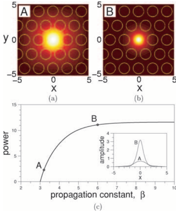
Figure 1. (a,b) Examples of stationary solutions for scalar PCF spatial solitons for \beta = 3.2 and \beta = 6 , and (c) power dependence of the soliton family. Points A and B in the power diagram (c) correspond to the examples (a,b), respectively. Inset: the corresponding one-dimensional profiles at y=0 for both examples.
