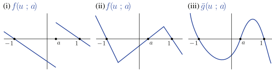
FIGURE 1. Panel (i) depicts the McKean caricature f(u; a) = \text{sign}(u - a) - u , while the piecewise linear zigzag nonlinearity considered in [12] is shown in panel (ii). Panel (iii) illustrates the assumption (Hg2) on \bar{g} . In the context of (1.1), we have \bar{g} = f .
