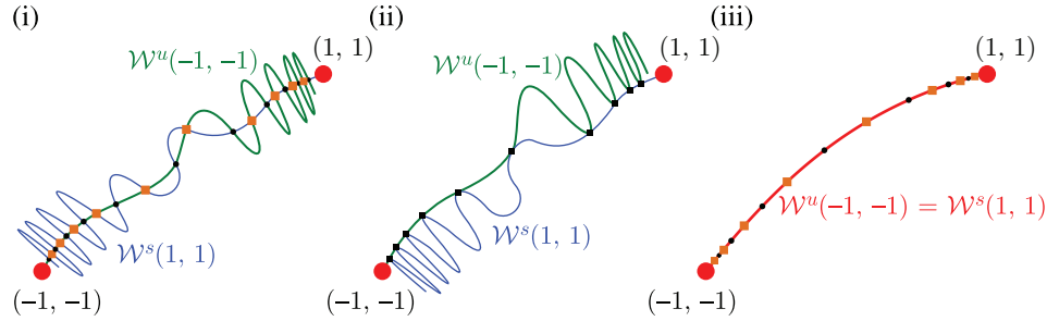
FIGURE 2. The stable and unstable manifolds \mathcal{W}^s(1, 1) and \mathcal{W}^u(-1, -1) associated to the discrete system (1.5) can intersect in several ways. Black circles are used to represent the site-centered solutions p^{(s)} and orange squares (online version only) are used for the bond-centered solutions p^{(b)} . In panel (i) the aforementioned manifolds intersect transversely, which means p^{(s)} and p^{(b)} will persist for a \approx 0 . Panel (ii) illustrates the saddle-node bifurcation at a = a_{\pm} that destroys these two branches of stationary solutions. Panel (iii) depicts the case covered by assumption (Hp). One can interpolate freely between p^{(s)} and p^{(b)} to find a one-parameter family of stationary solutions p^{(v)} to (1.10) at a = 0 .
