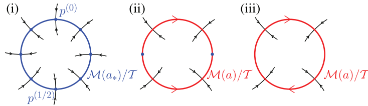
FIGURE 3. Panel (i) depicts the manifold \mathcal{M}(a_*) after factoring out the symmetry \mathcal{T} . Each point on the circle represents an equivalence class p^{(\vartheta)} with \vartheta \in S^1 . We show that \mathcal{M}(a_*) is normally hyperbolic and that it persists as \mathcal{M}(a) for a near a_* . As illustrated in panel (ii), one or more of the equilibria can survive for a \neq a_* , in which case (1.10) suffers from propagation failure. However, if (1.10) is a normal family, the flow on \mathcal{M}(a) must behave as shown in panel (iii), inducing travelling wave solutions to (1.10).
