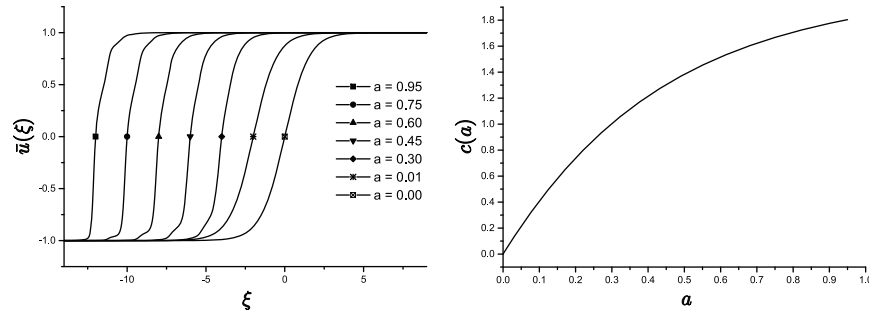
FIGURE 5. Selected wave profiles and wave speed plot for (3.1) with the nonlinearity g = g_2 defined in (3.8). As in Example 1, no propagation failure occurs and the wave profiles \bar{u} remain smooth as a \rightarrow 0 .
