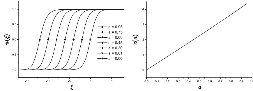
FIGURE 4. Selected wave profiles and wave speed plot for (3.1) with the nonlinearity g = g_1 defined in (3.6). No propagation failure occurs, and the wave profiles \bar{u} remain smooth as a \rightarrow 0 .
