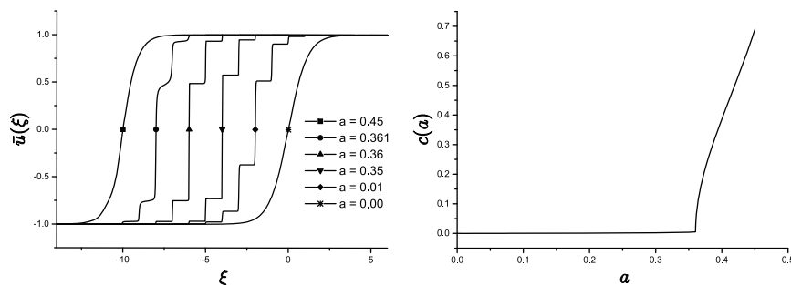
FIGURE 6. Selected wave profiles and wave speed plot for (3.1) with the nonlinearity g = g_3 defined in (3.9). Despite the smooth profile of the wave at a = 0 , propagation failure occurs and the wave profiles are step functions for 0 < a < a_+ \approx 0.36025 .
